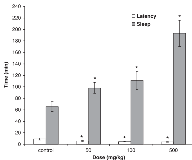
Figure 1. Effect of ETC administration on the latency to sleep and sleeping time (min) induced by pentobarbital (50 mg/kg). Data are presented as mean \pm SEM ( n = 10 ). * p < 0.05 compared with control group, ANOVA/Duncan.
